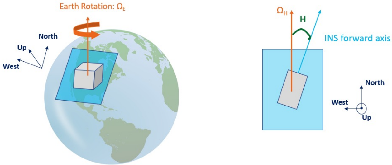
Figure 4: Heading definition: The heading is the angle between the forward axis and the North direction, defined as the Earth rotation vector projected in the horizontal frame
