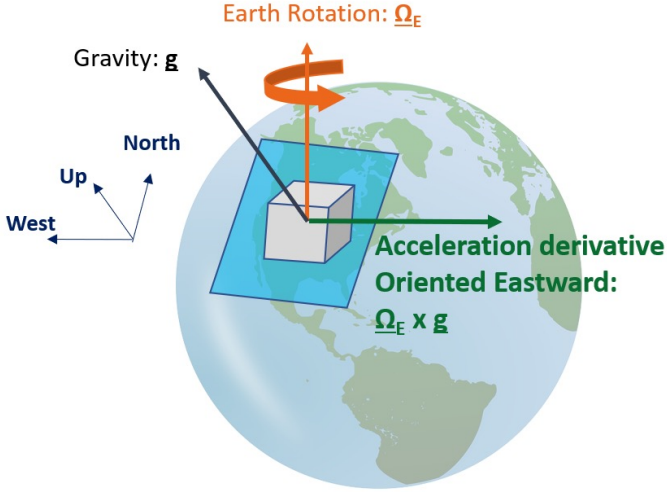
Figure 10: The East direction is provided by the derivative of the acceleration
