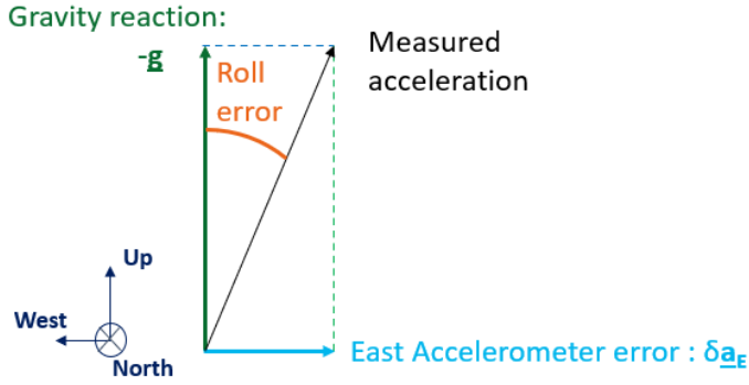
Figure 2: Impact of an accelerometer error on the roll error
