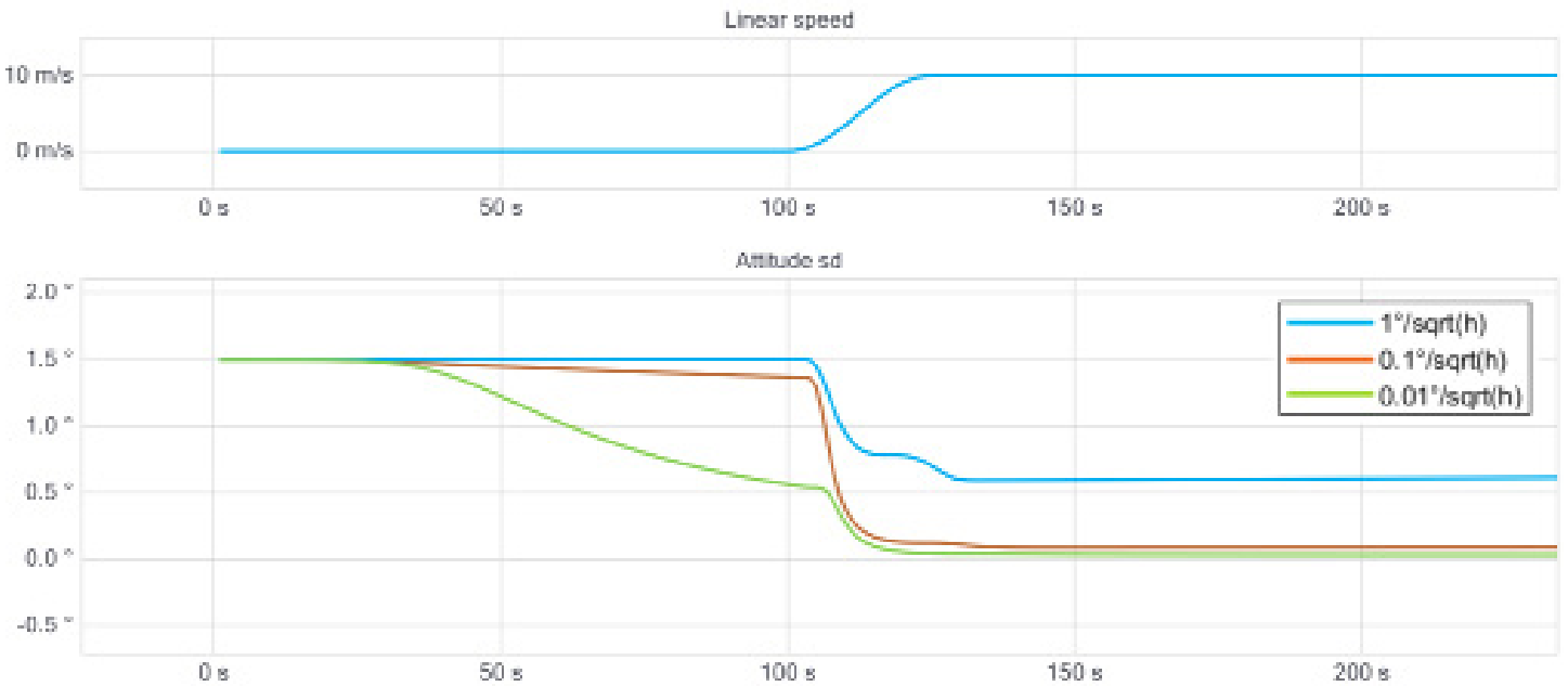
Figure 20: Heading standard deviation with varying gyro noise
