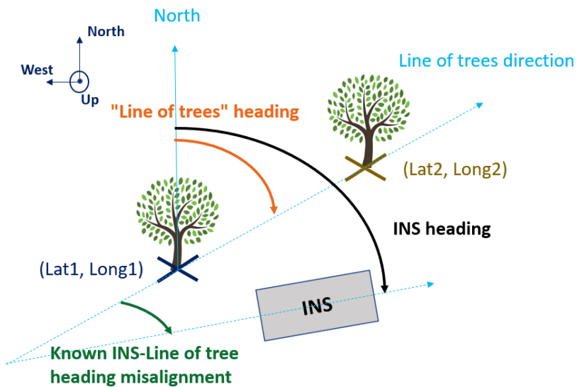
Figure 15: The heading of the INS can be determined using 2 features and the known misalignment between the features and the INS
