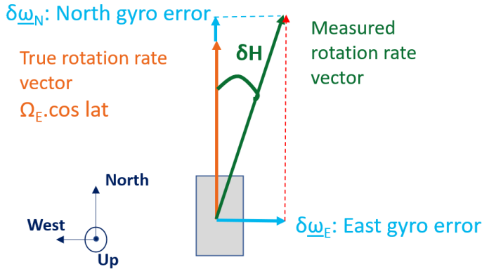
Figure 7: Impact on a gyro bias on the heading estimation
