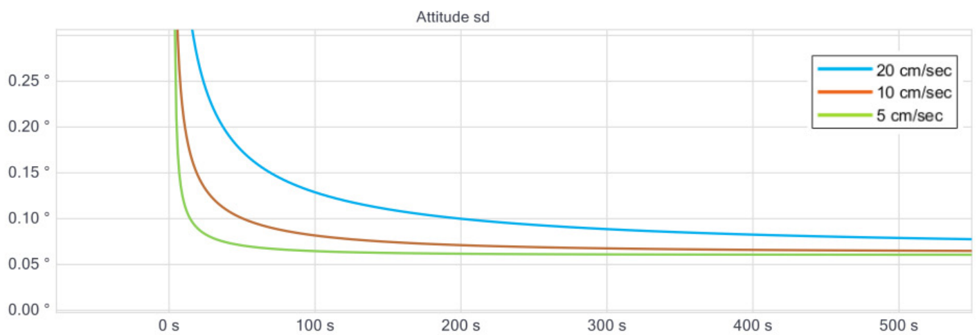
Figure 25: Heading standard deviation with varying gyro noise
