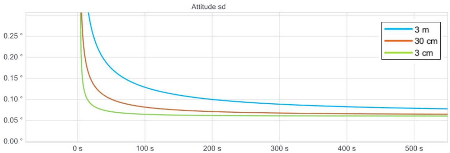
Figure 26: Heading standard deviation with varying GNSS noise
