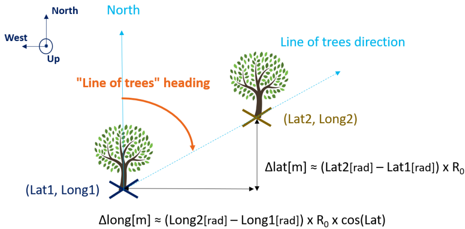
Figure 14: Heading of a direction defined by 2 positions - In this figure, the Earth is considered spherical with Radius R_0 , and that the difference of latitude between the 2 points is small. Lat = 0.5 \times (Lat1 + Lat2)
