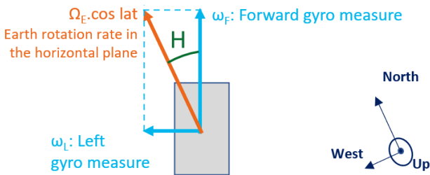
Figure 6: Measuring the Earth rotation to determine the heading
