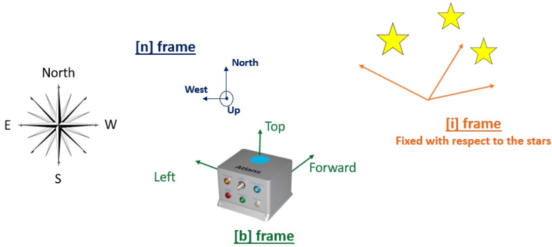
Figure 9: Frames definition
