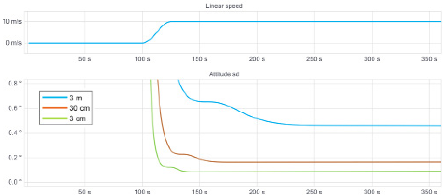
Figure 22: Heading standard deviation with varying GNSS noise
