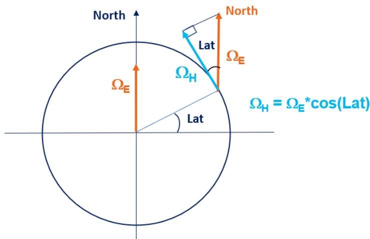
Figure 5: Projection of the Earth rotation rate in the horizontal frame
