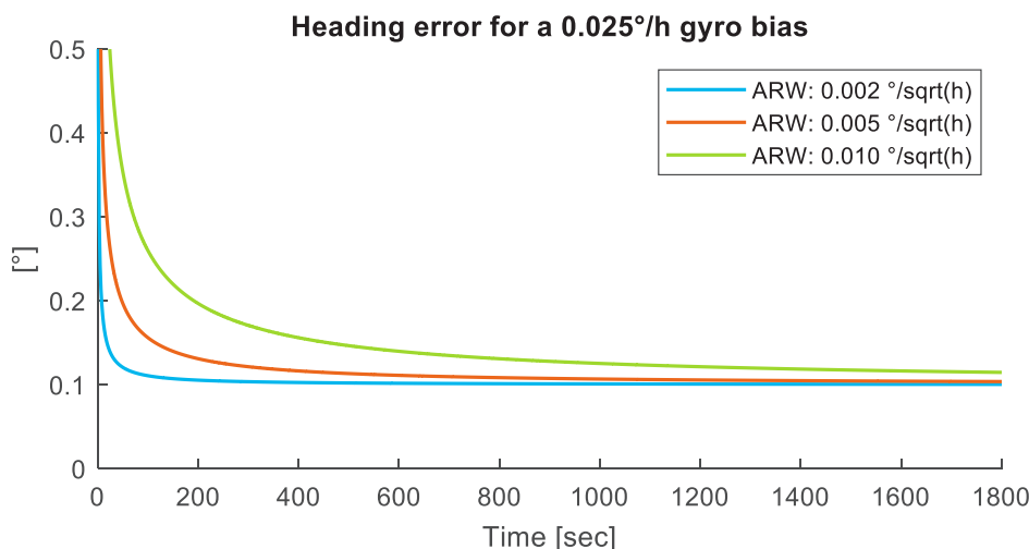
Figure 13: Heading accuracy convergence time
