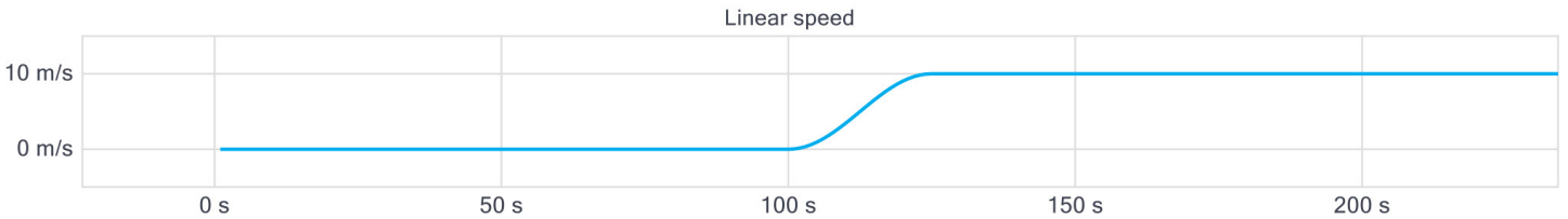
Figure 19: Dynamic profile of the test trajectory: forward speed
