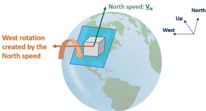
Figure 8: A North speed creates a Westward rotation
