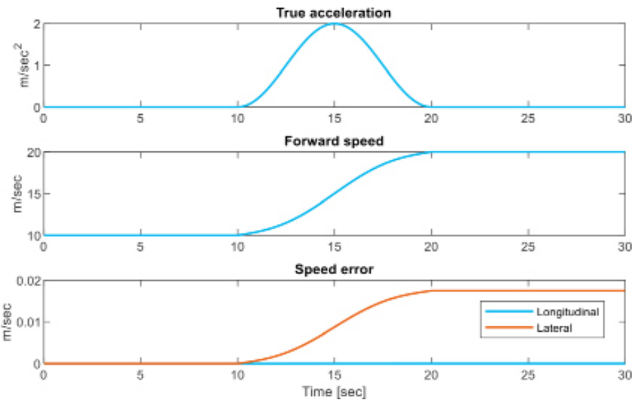
Figure 18: Impact of the heading error on the speed in case of acceleration - The image illustrates the impact of a 0.1° heading error. When the system accelerates from 10 to 20m/sec, a lateral speed of 0.017m/sec is created in the lateral direction (i.e., the direction orthogonal to the acceleration)
