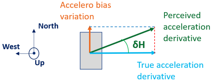
Figure 12: Impact of an accelerometer bias variation
