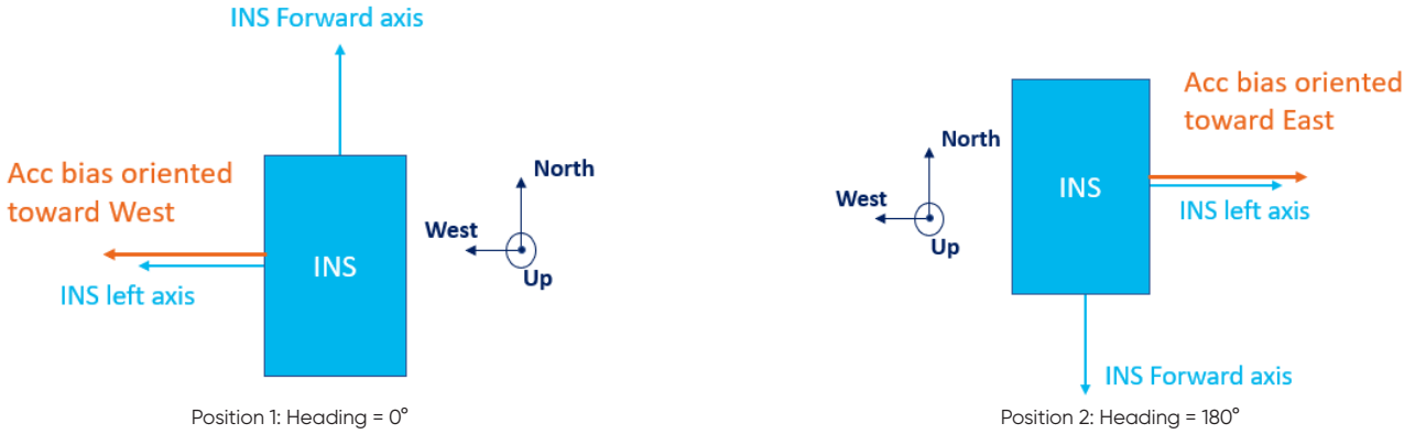
Figure 3: 2-position static alignment
