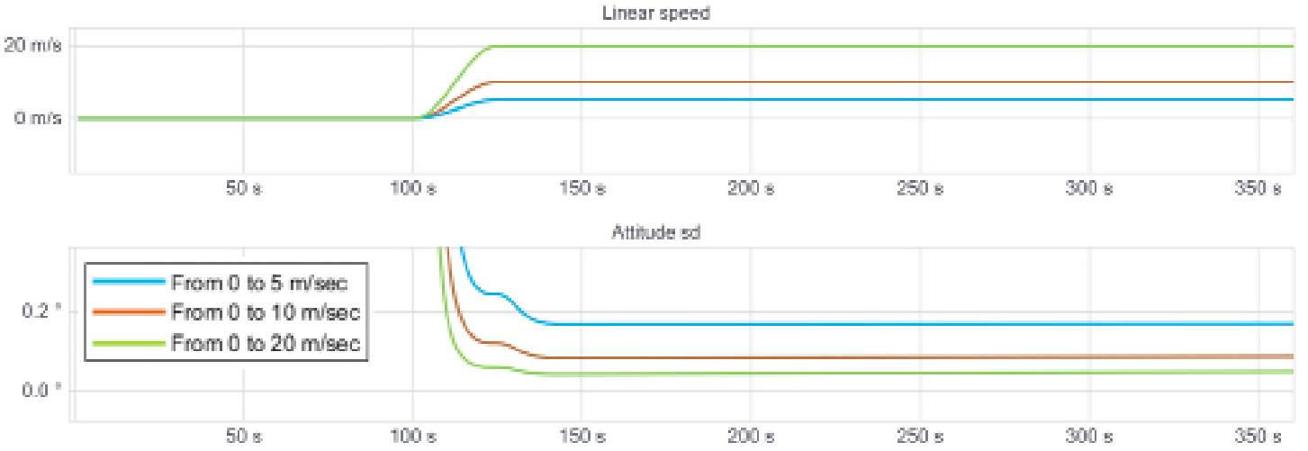
Figure 23: Heading standard deviation with varying acceleration
