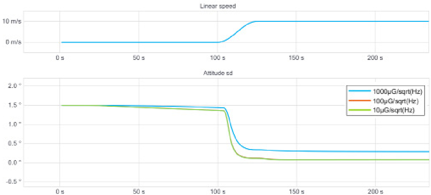
Figure 21: Heading standard deviation with varying gyro noise
