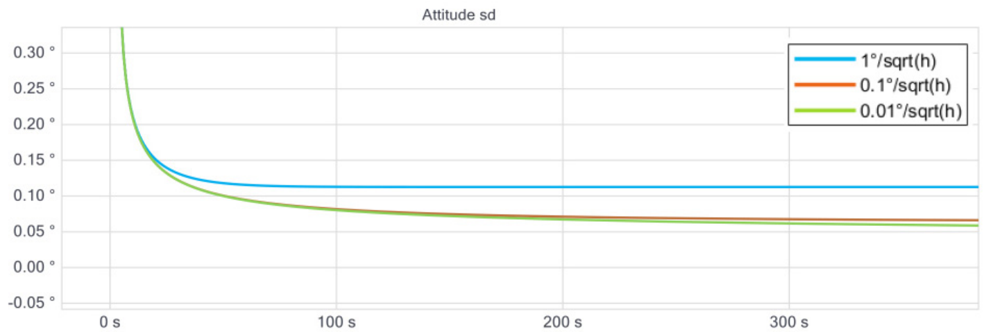
Figure 24: Heading standard deviation with varying gyro noise
