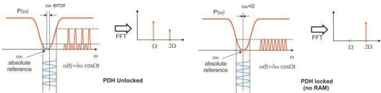
Figure 11: PDH representation without RAM taken into account
