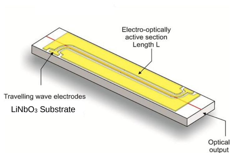
Figure 1: Phase Modulator diagram
