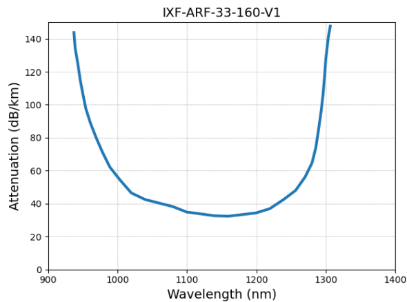
Typical attenuation of IXF-ARF-33-160-V1 fiber optimized for operation around 1 \mu m.
