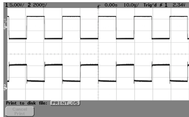
Figure 4: up: modulation signal at 50 kHz down: resulting intensity signal
